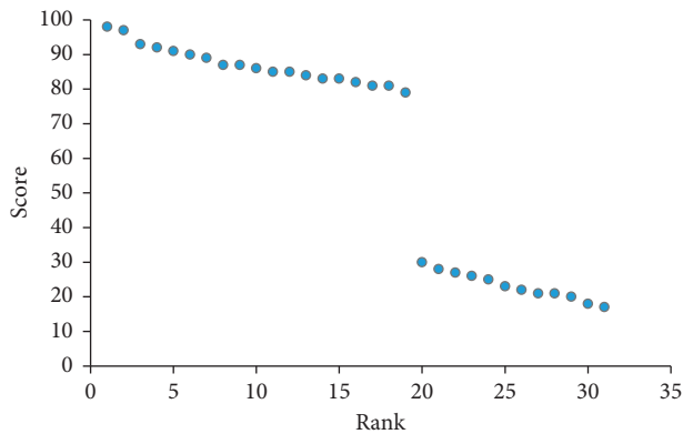
FIGURE 6: Divide in WD data set.
